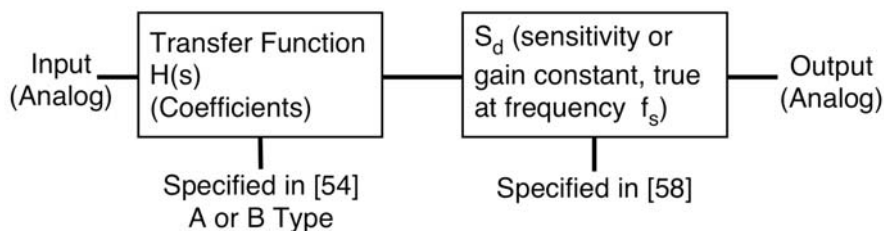
Figure 7: Example Analog Stage Using Coefficients Representation
