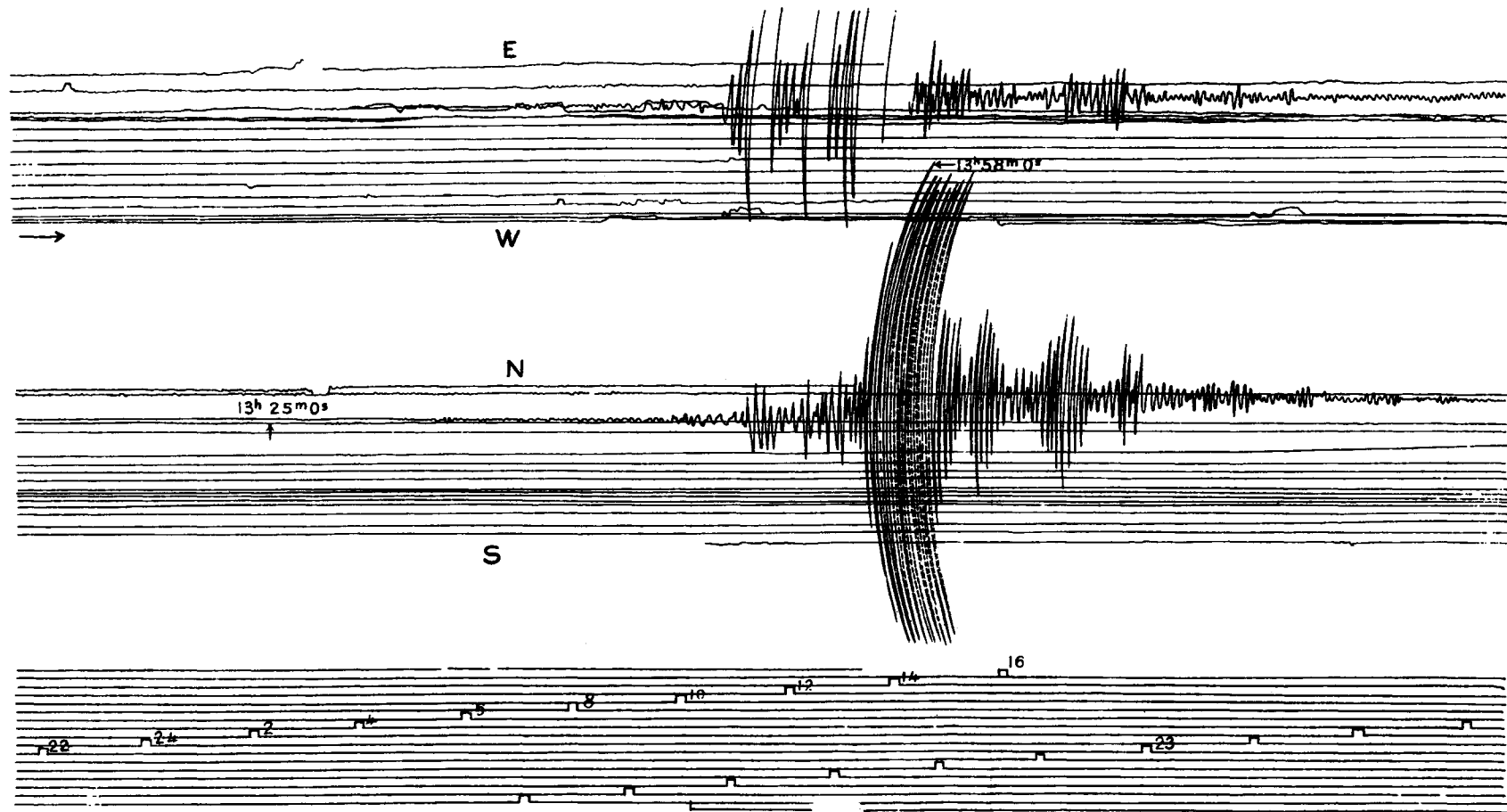
SHIDE, ISLE OF WIGHT, ENGLAND. Heavy Horizontal Pendulum. (From half-tone reproduction; reduced \frac{1}{16} .)
