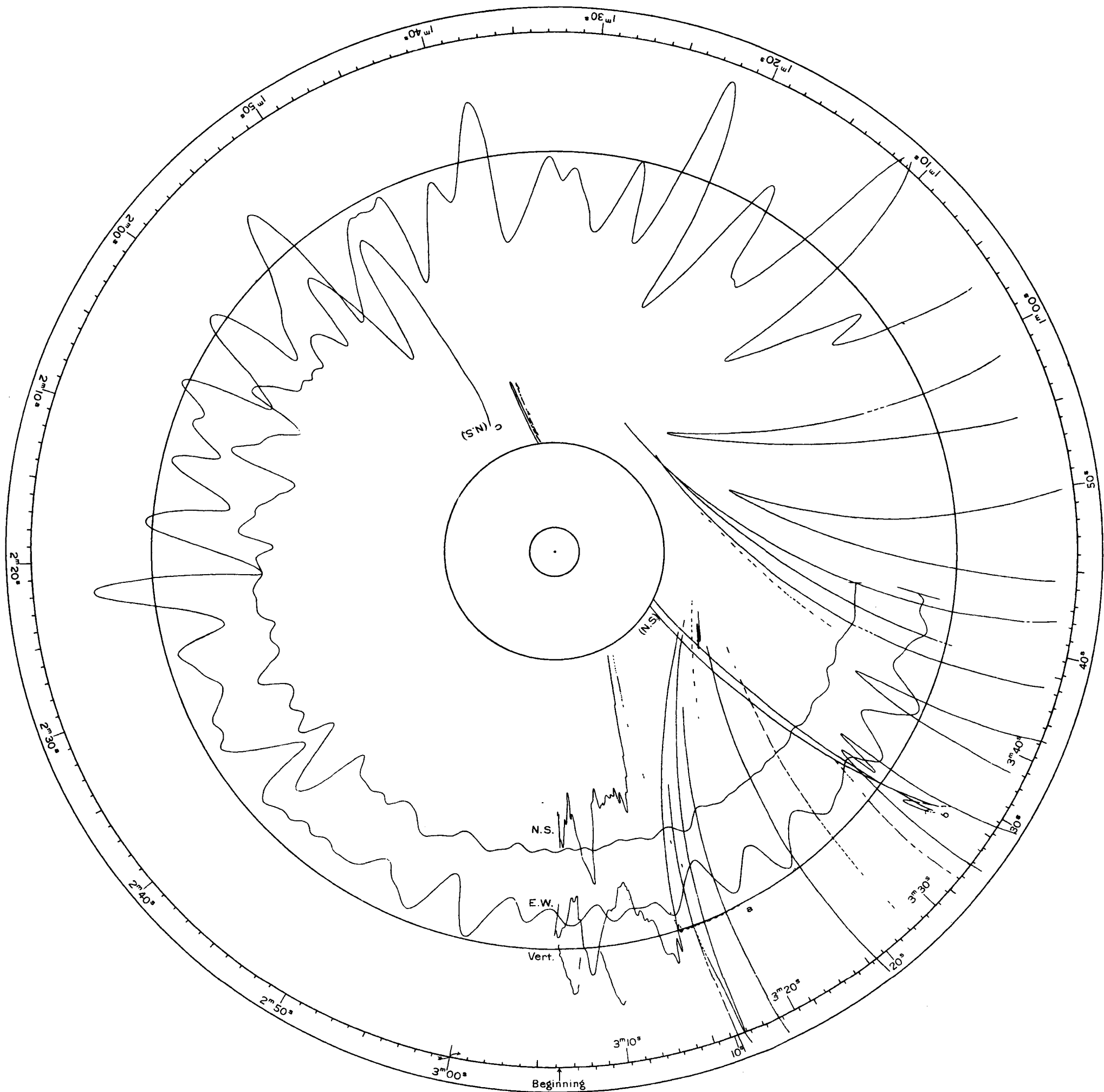
MT. HAMILTON, CAL. Ewing Three-Component Seismograph. (From hand-tracing; reduced 1:2.)
