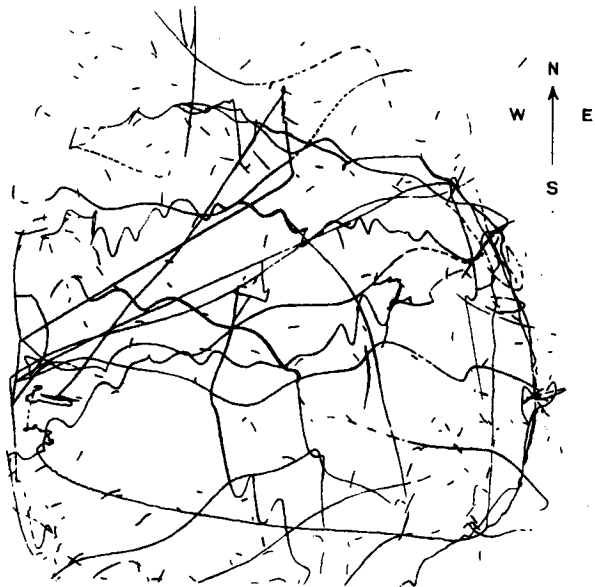
ALAMEDA, CAL. Ewing Duplex Pendulum. (From blue-print.)
