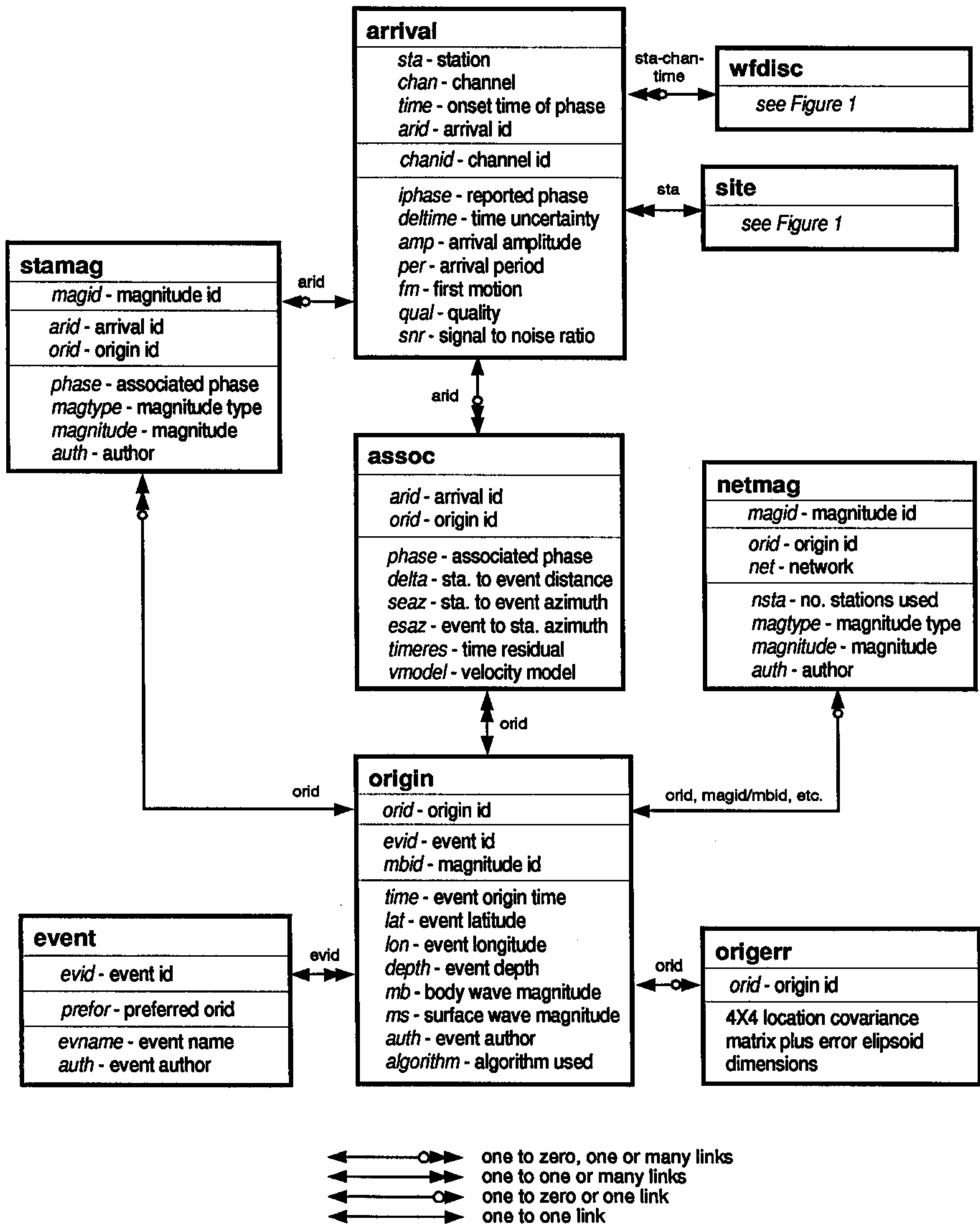
Figure 2. Database schema map for JSPC information products. Event related tables.
