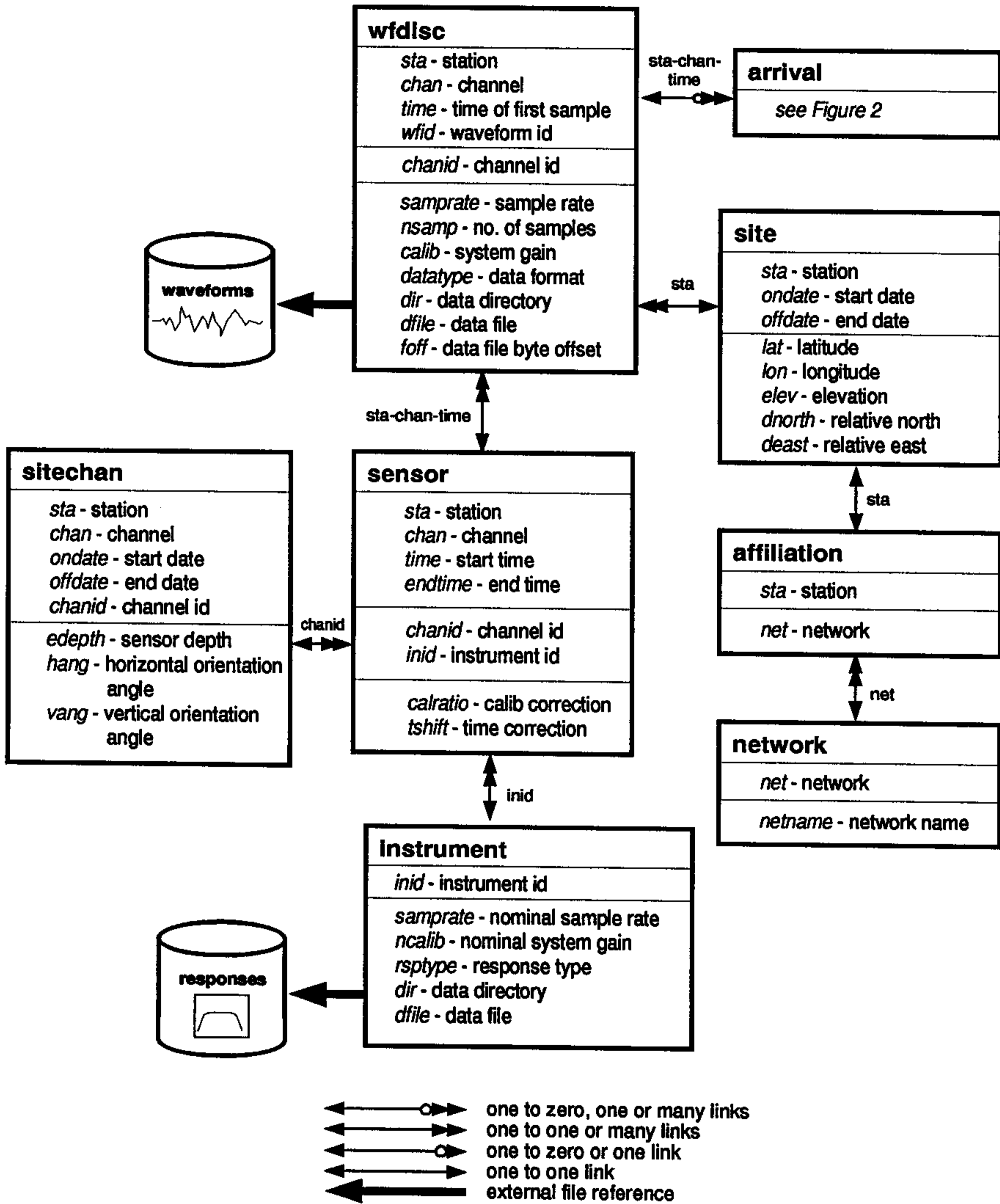
Figure 1. Database schema map for JSPC information products. Waveform data tables.
