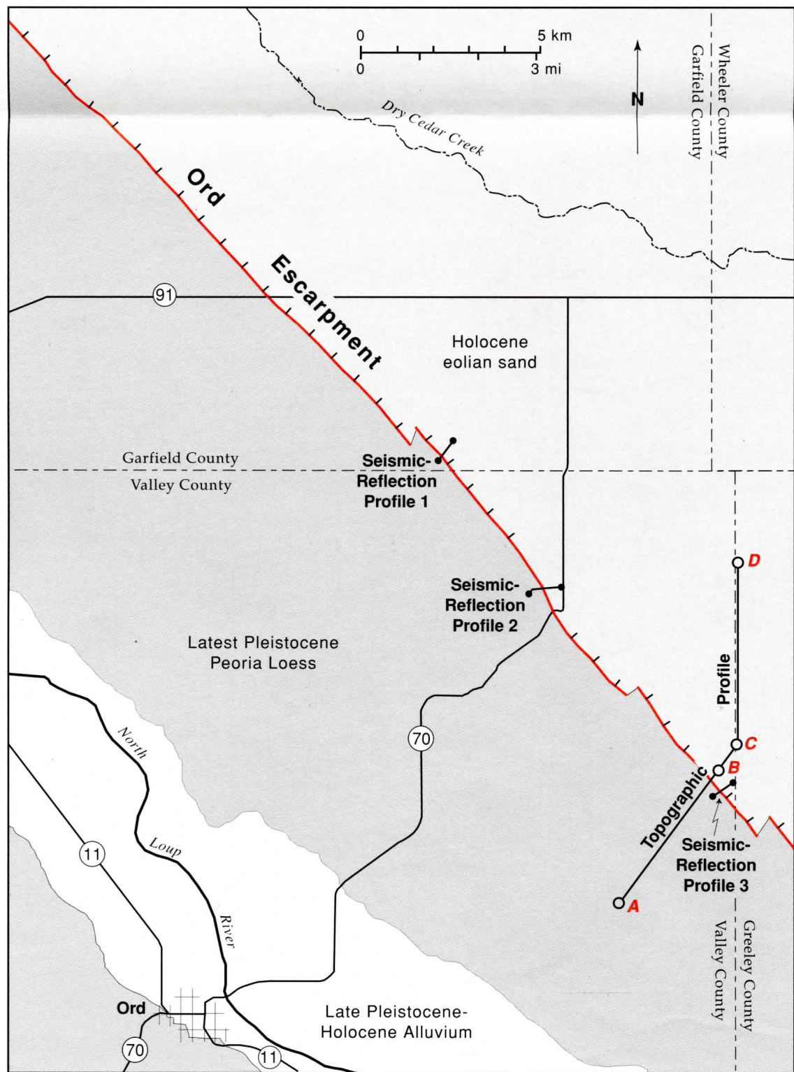
Figure 2. Location map of the Ord escarpment showing distribution of Peoria Loess, Holocene eolian sand, and locations of seismic-reflection profiles. Black hachures on red escarpment point toward lowlands. Open circles show locations of drill holes. Topographic profile and shallow subsurface stratigraphy are shown in figure 3
